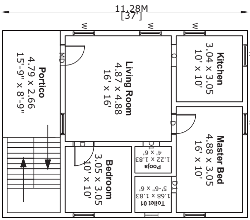
SITE CUM PRO. GROUND FLOOR PLAN
