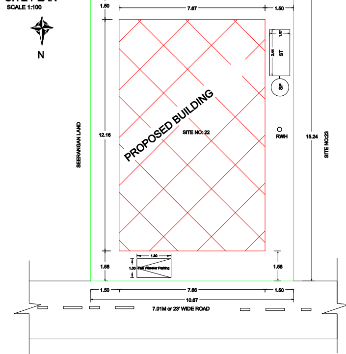
SITE PLAN
