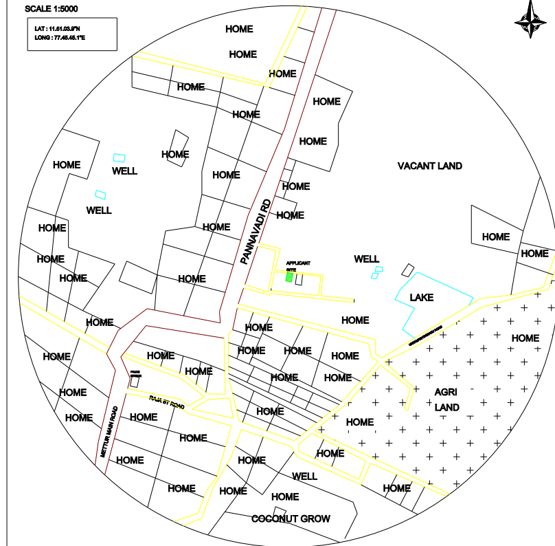
TOPO PLAN
