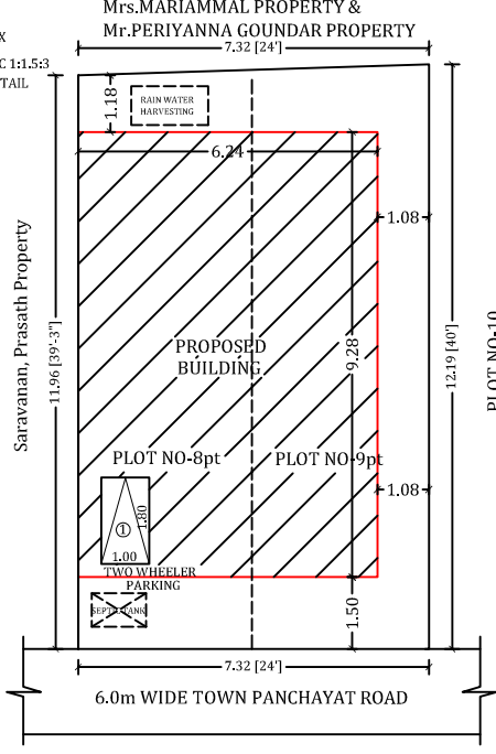
SITE PLAN
