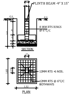
COLUMN & FOOTING DETAIL
