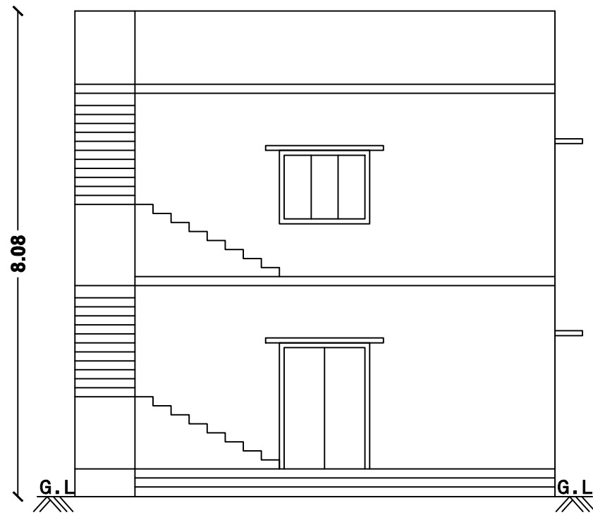
FRONT ELEVATION
