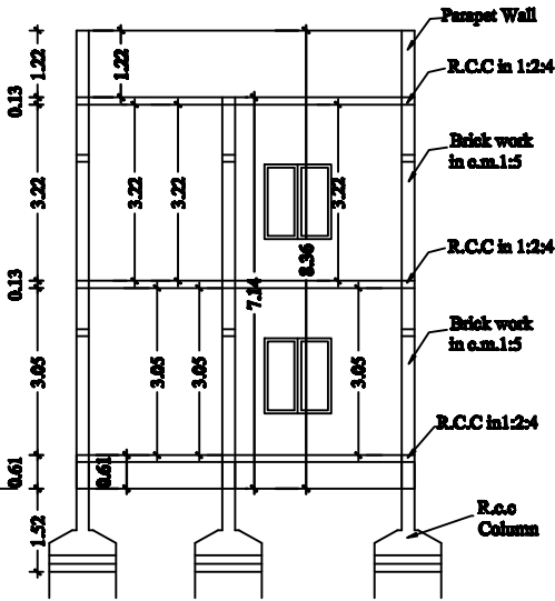
CROSS SECTION-AA
