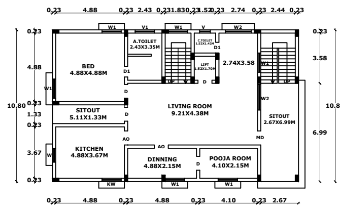
EXISTING GROUND FLOOR
