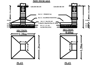
COLUMN FOOTING DETAILS
