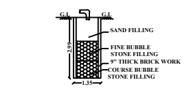
SECTION ON RAIN WATER COLLECTION TANK
