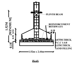
TYP.DET. COLUMN FOOTING
