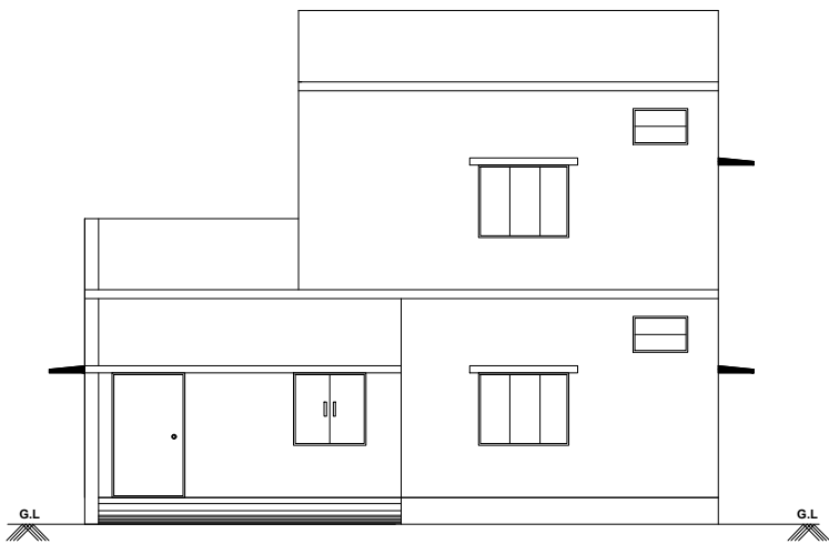
FRONT ELEVATION
