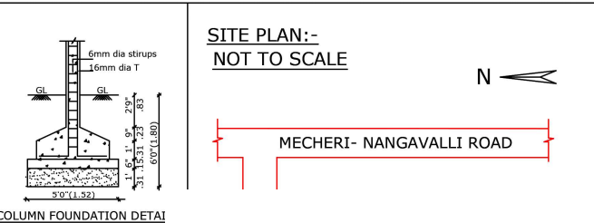
COLUMN FOUNDATION DETAIL
