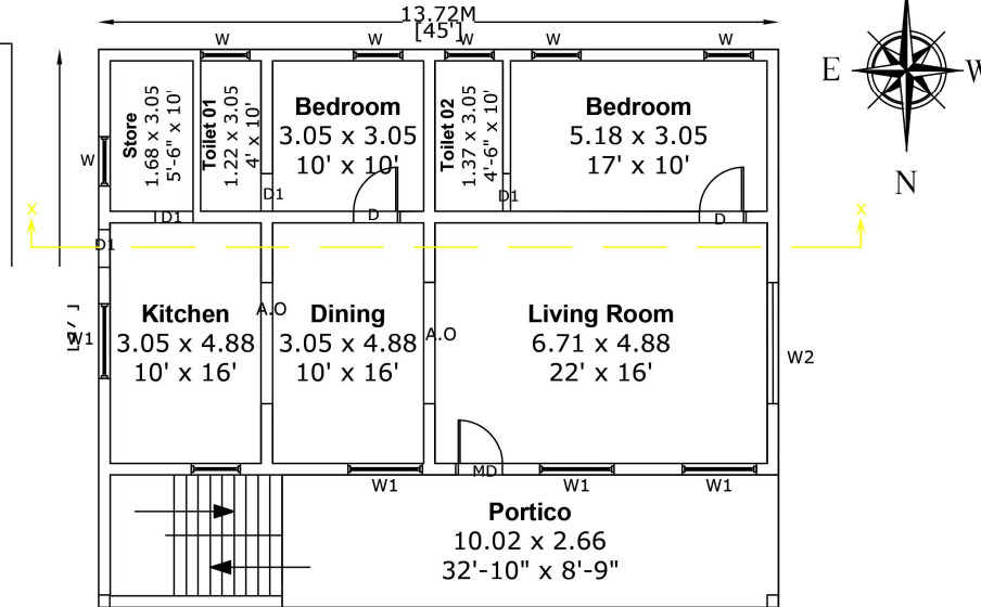
SITE CUM PRO. GROUND FLOOR PLAN
