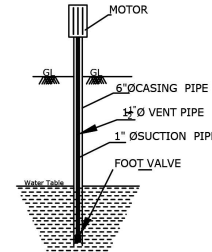
SEC. OF BOREWELL
