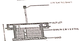
SECTION OF THE SEPTIC TANK
