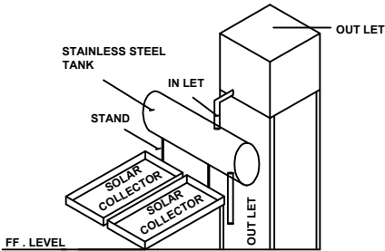
SOLAR HEATING WATER SYSTEM
