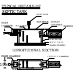
LONGITUDINAL SECTION SEPTIC TANK
