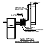
DETAILS OF RAIN WATER HARVESTING TANK
