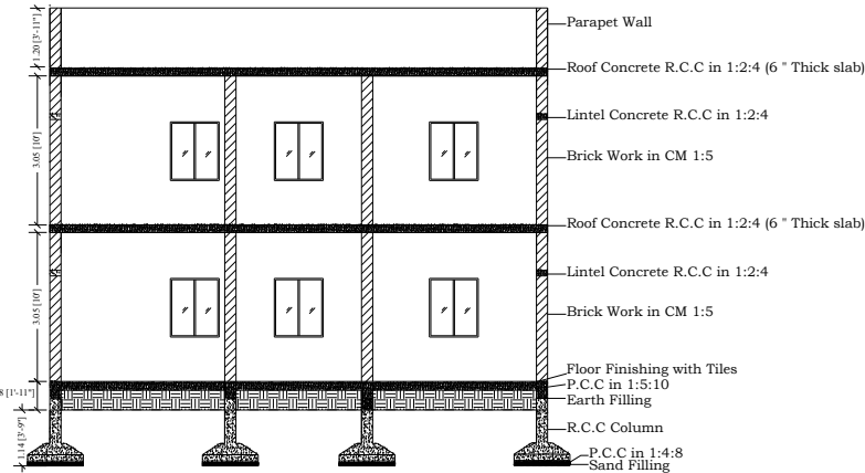
SECTION X-X
