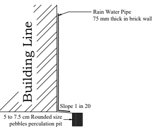
RAINWATER HARVESTING
