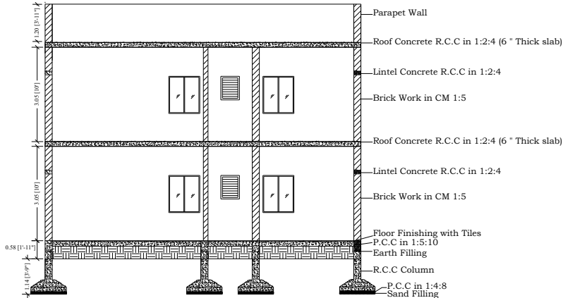
SECTION X-X
