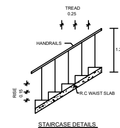
STAIRCASE DETAILS
