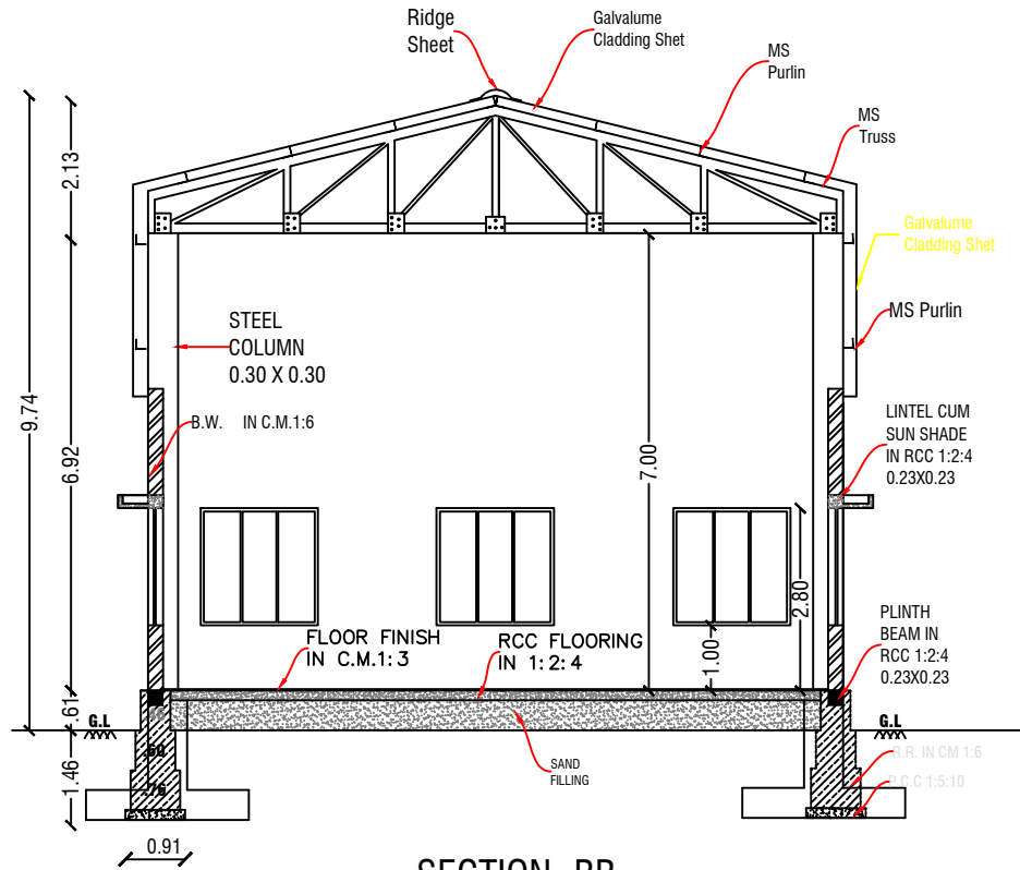
SECTION -BB
