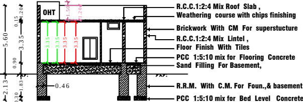
SECTION ON "XY"
