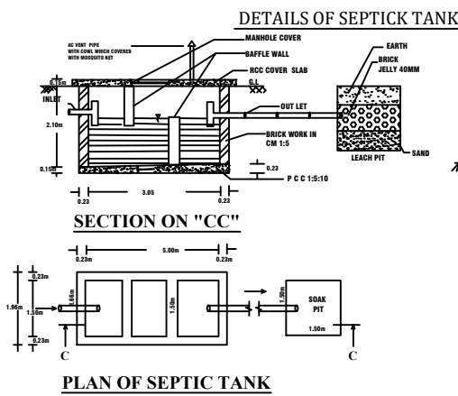
PLAN OF SEPTICK TANK
