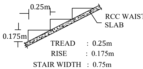
PRO. STAIRCASE DETAIL (NOT TO SCALE)
