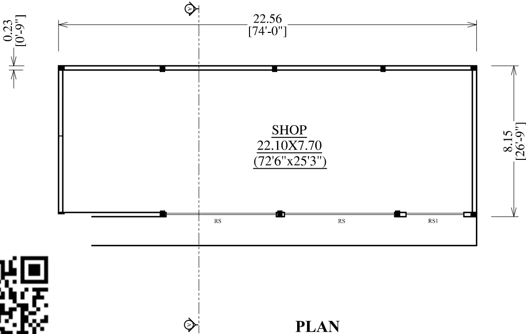
PLAN FACED TO SOUTH
