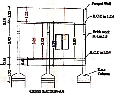
CROSS SECTION-AA
