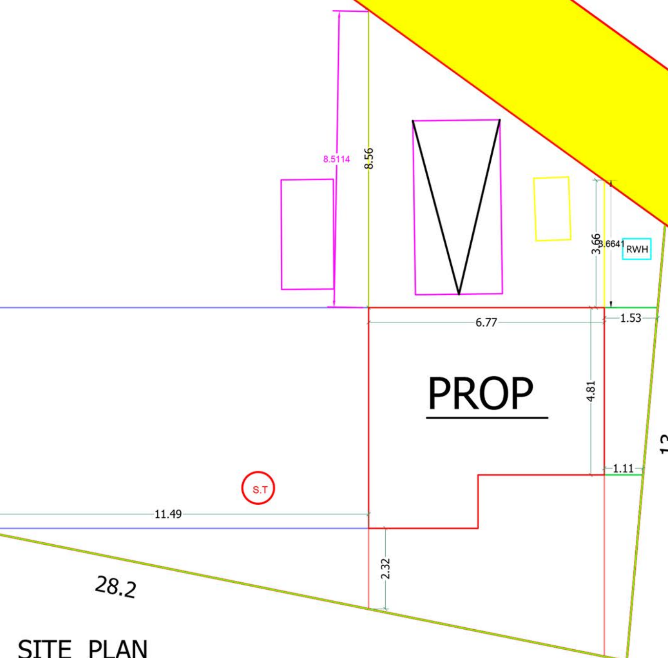
SITE PLAN
