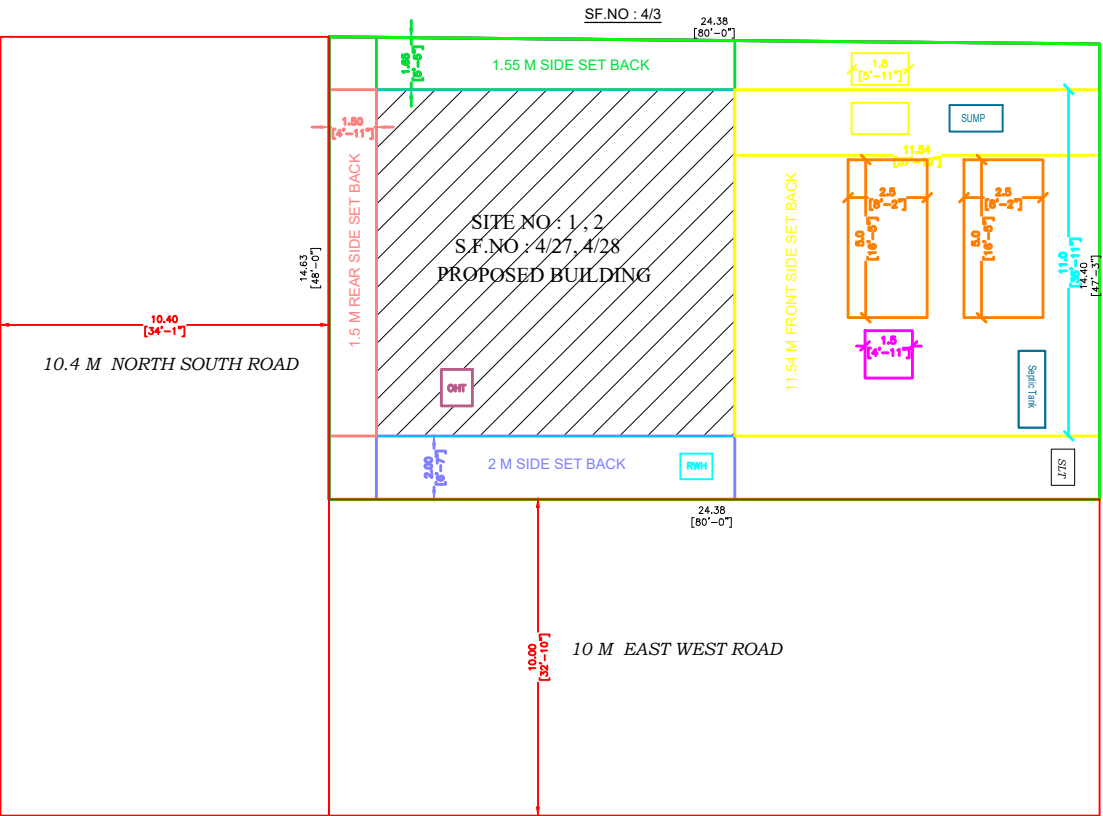
SITE PLAN
