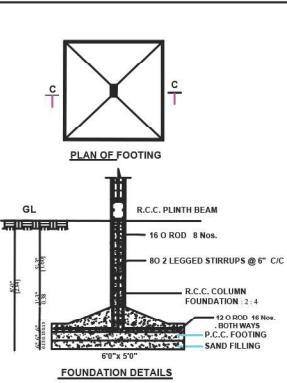
FOUNDATION DETAILS
