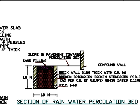
SECTION OF RAIN WATER PERCOLATION BED
