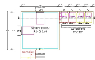
GROUND FLOOR PLAN SCALE 1: 100 BLOCK-2
