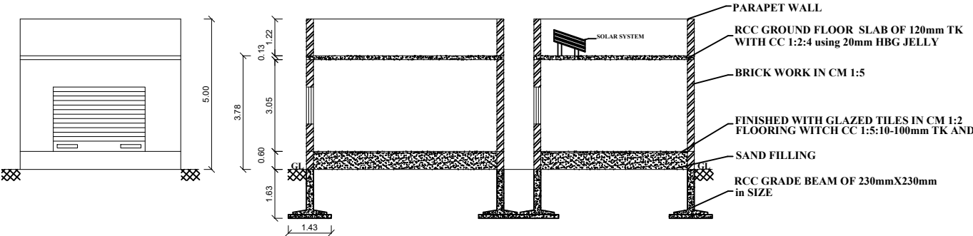
FRONT ELEVATION
