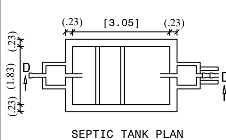
SEPTIC TANK PLAN
