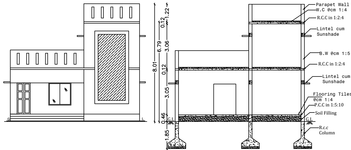
FRONT ELEVATION
