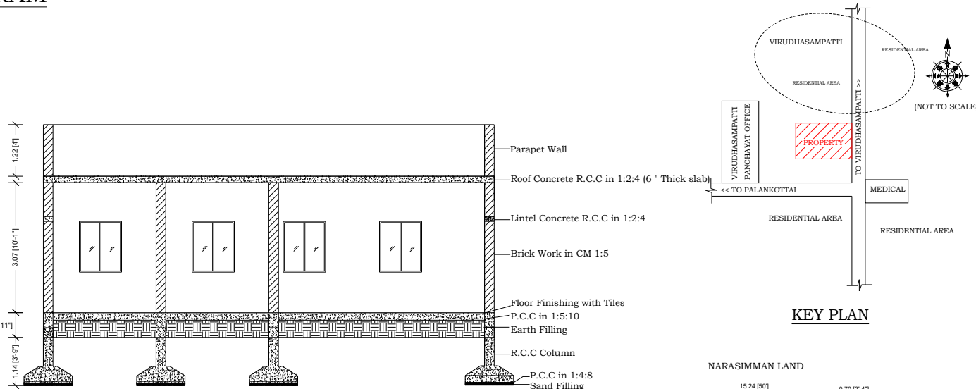
SECTION X-X
