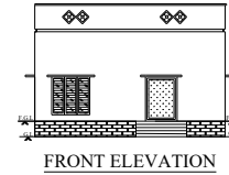
FRONT ELEVATION
