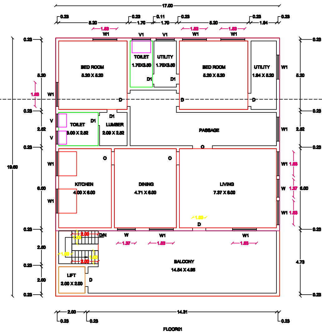
FLOOR-1
