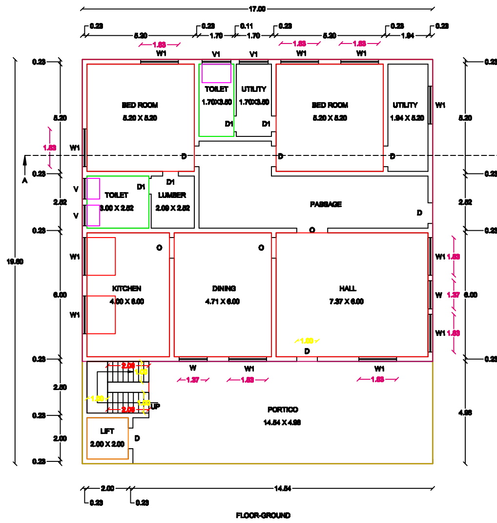
FLOOR-GROUND
