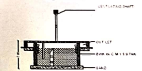
SEPTIC TANK
