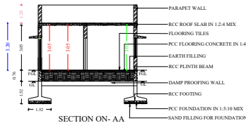
SECTION ON-AA
