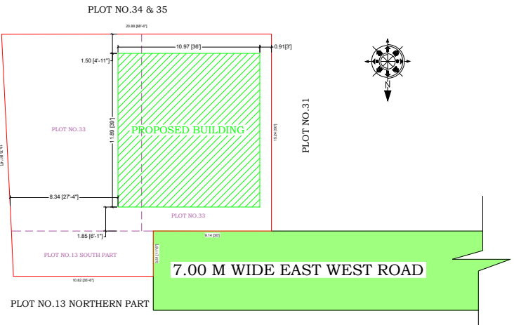
SITE PLAN (SCALE -1:250)
