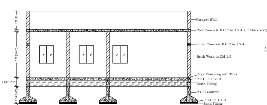
SECTION X-X
