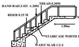
STAIRCASE DETAILS
