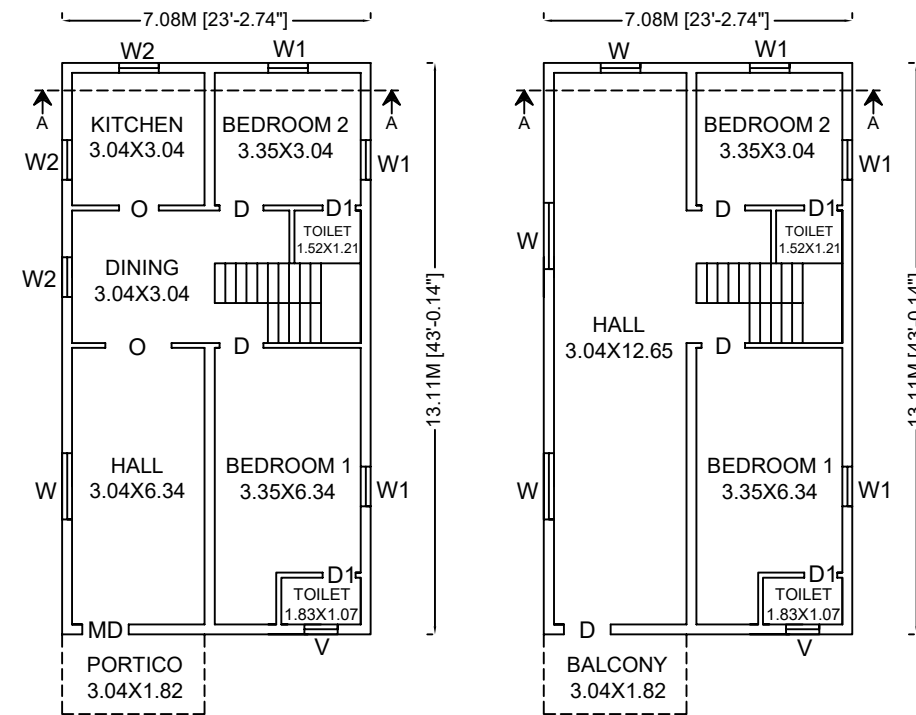
GROUND FLOOR PLAN FIRST FLOOR PLAN
