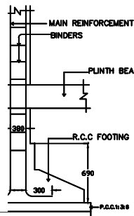
TYPICAL SECTION OF R.C.C COLUMN FOUNDATION SCALE : 1"=2'-0"
