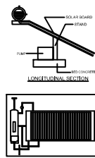
SOLAR WATER HEATER
