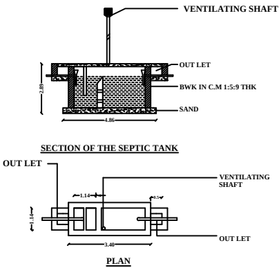
SEPTIC TANK
