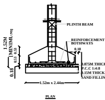
YP.DET. COLUMN FOOTING
