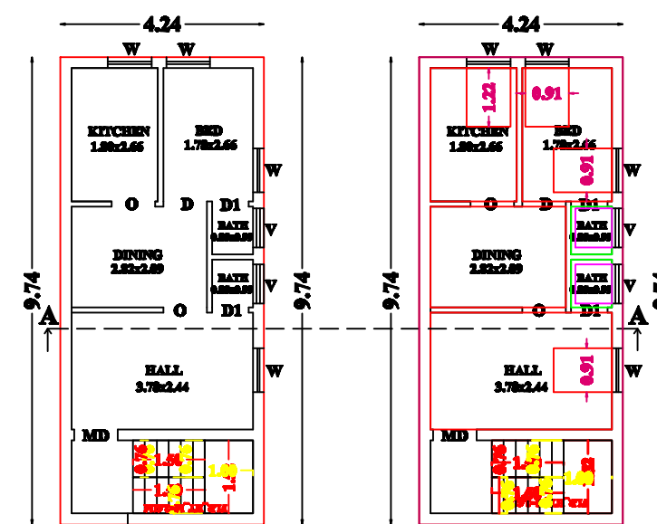
GROUND FLOOR PLAN (EXISTING)
