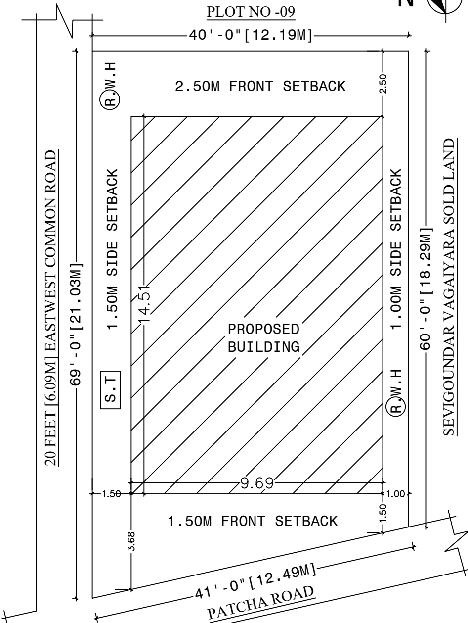
SITE PLAN (1:100)
