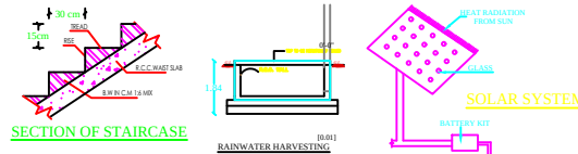
RAINWATER HARVESTING
