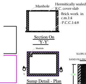
Sump Detail - Plan
