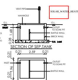
SECTION OF SEPTIC TANK
