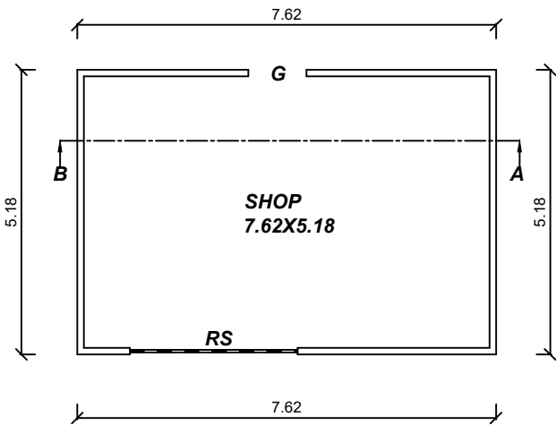
ROUND FLOOR PLAN
