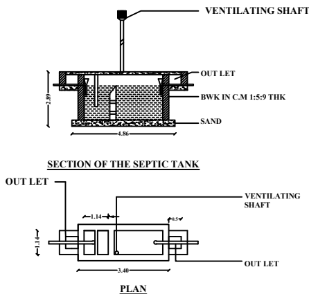
SEPTIC TANK
