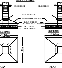
COLUMN FOOTING DETAILS
