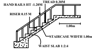
STAIRCASE DETAILS
