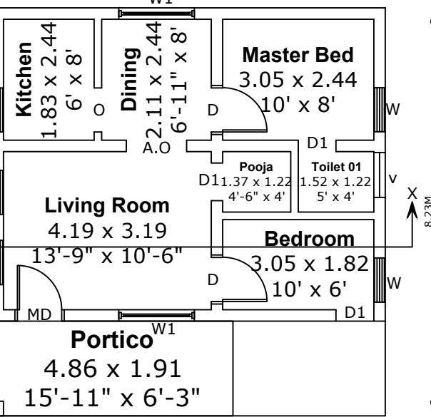
SITE CUM PRO.GROUND FLOOR
