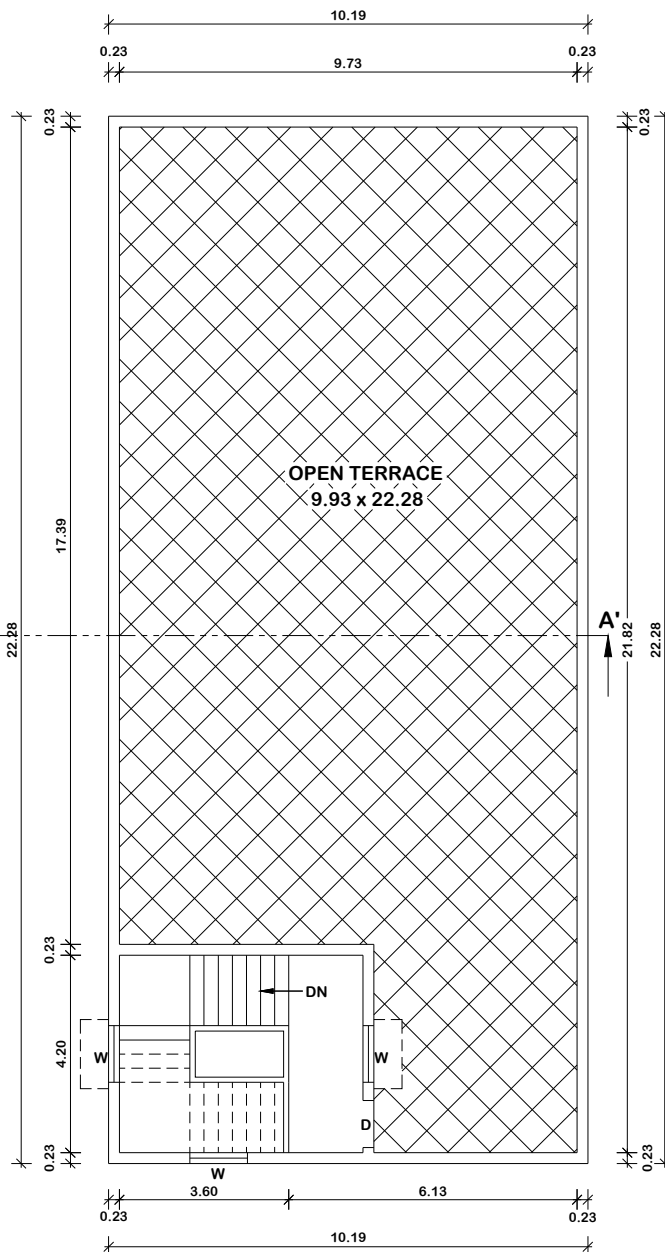
TERRACE FLOOR
