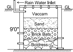
RAIN WATER HARVESTING TANK
