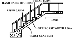
STAIRCASE DETAILS
