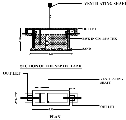
SEPTIC TANK
